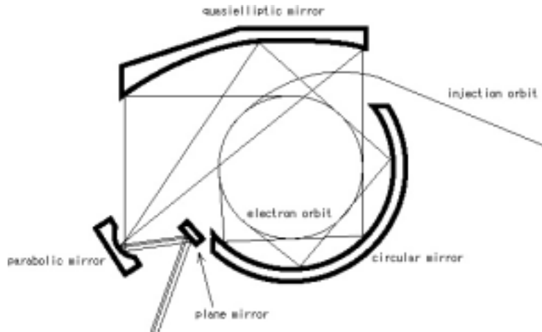
FIGURE 3. The special mirror system is composed of the circular mirror concentric to the electron orbit, quasi-elliptic mirror, which focuses the radiation in to one point, parabolic mirror which makes parallel beam to be extracted.
