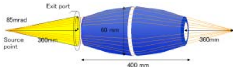
FIGURE 4. Eight sets of multi-layer cylindrical mirrors will be made by the replica method. Mother body must have the surface roughness less than nm and the shape tolerance less than 1 \mu \text{ m} .
