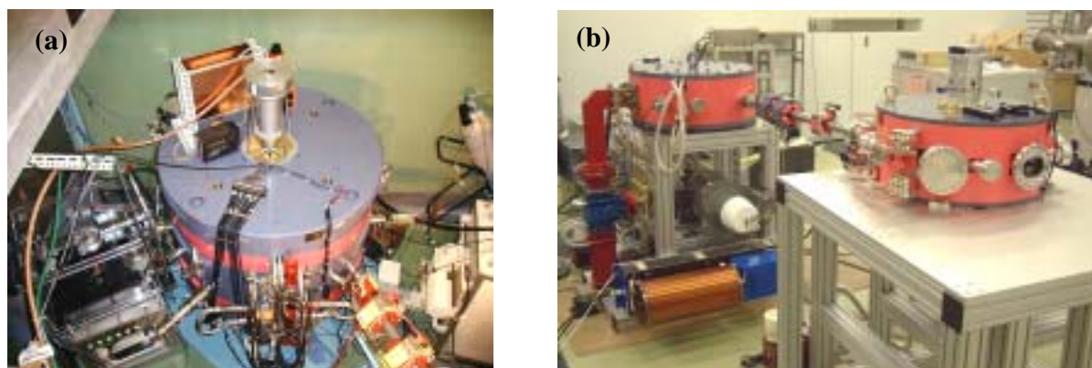
FIGURE 2. MIRRORCLE-20 (left) and MIRRORCLE-6X (right) are the portable exact circular synchrotrons using normal conducting magnet.
