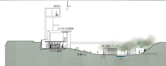
c-c' section S=1/300
