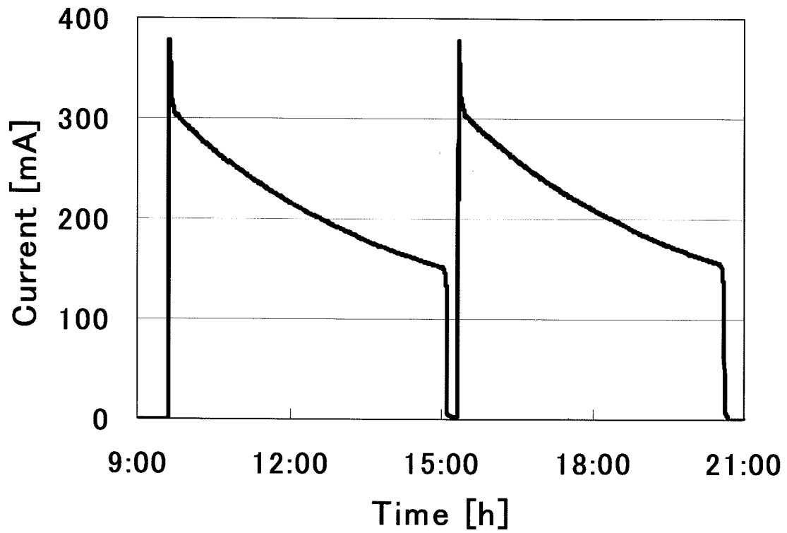
Fig.2. Typical variation in the accumulated electron beam current in a day.
