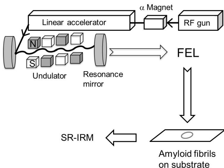
Figure 1. Schematic of the FEL and analysis setup. The laser beam is generated using an electronic gun and accelerated to 40 MeV by the linear accelerator. The periodic length of the undulator can be tuned to set the oscillation wavelength. The FEL beam is transported to the laboratory through a vacuum tube, and the irradiation to the sample on the substrate is controlled by a gold-coated mirror. After irradiation, the sample was analyzed using SR-IRM.
