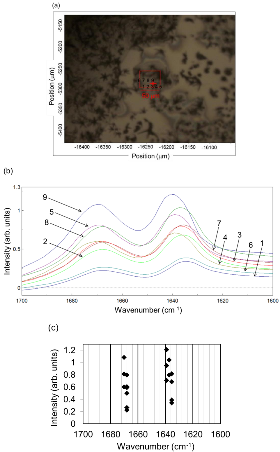
Figure 2. (a) SR-IRM image of the DFNKF amyloid fibrils before FEL irradiation. The target size was 50 \mu\text{m} \times 40 \mu\text{m} . The numbers (no.1-9) indicate the positions for measurements of spectra. (b) IR reflection spectra. (c) Plot of the peaks in the amide I region
