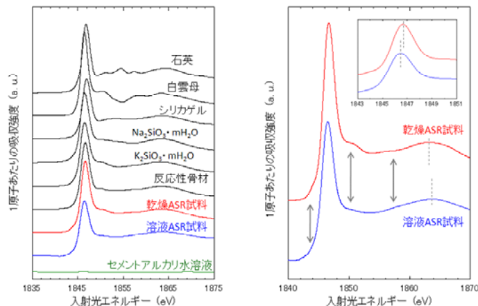
Fig.1. Observed Si K-edge XANES Spectra
