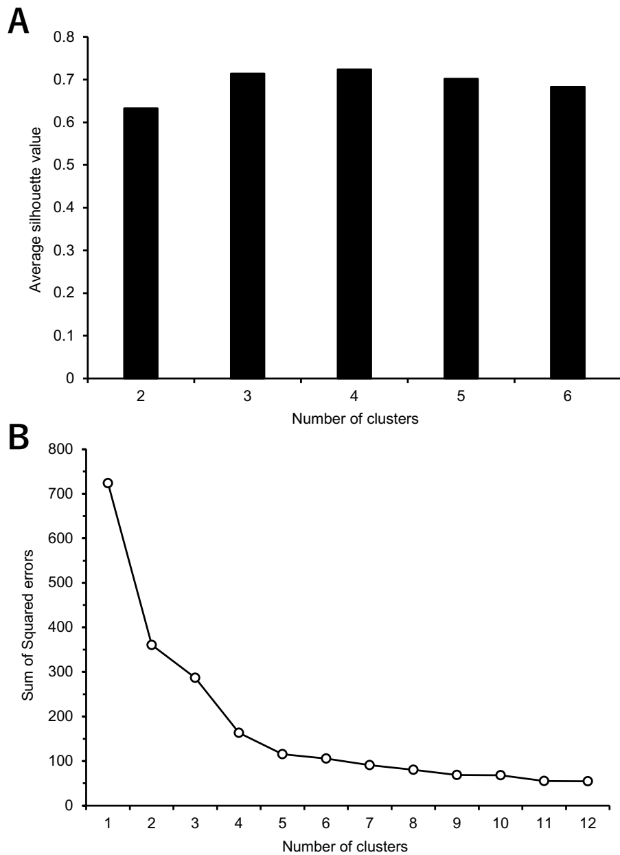
Figure 3-1. Average silhouette (A) and elbow (B) methods for K-means clustering analysis
